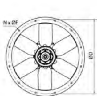
TGT short casing
