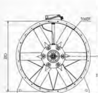
TGT 1400 and TGT 1600 long casing (LP)
