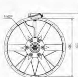
TGT 1400 and TGT 1600 Short casing
