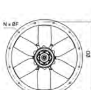
TGT ATEX-400 to TGT ATEX-1250 long casing (LP)
